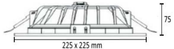
Cut-Out 200 x 200 mm
